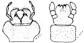
Fig. 128. Labium: a, Perla hastata Banks; b, Nemoura venosa Banks.
